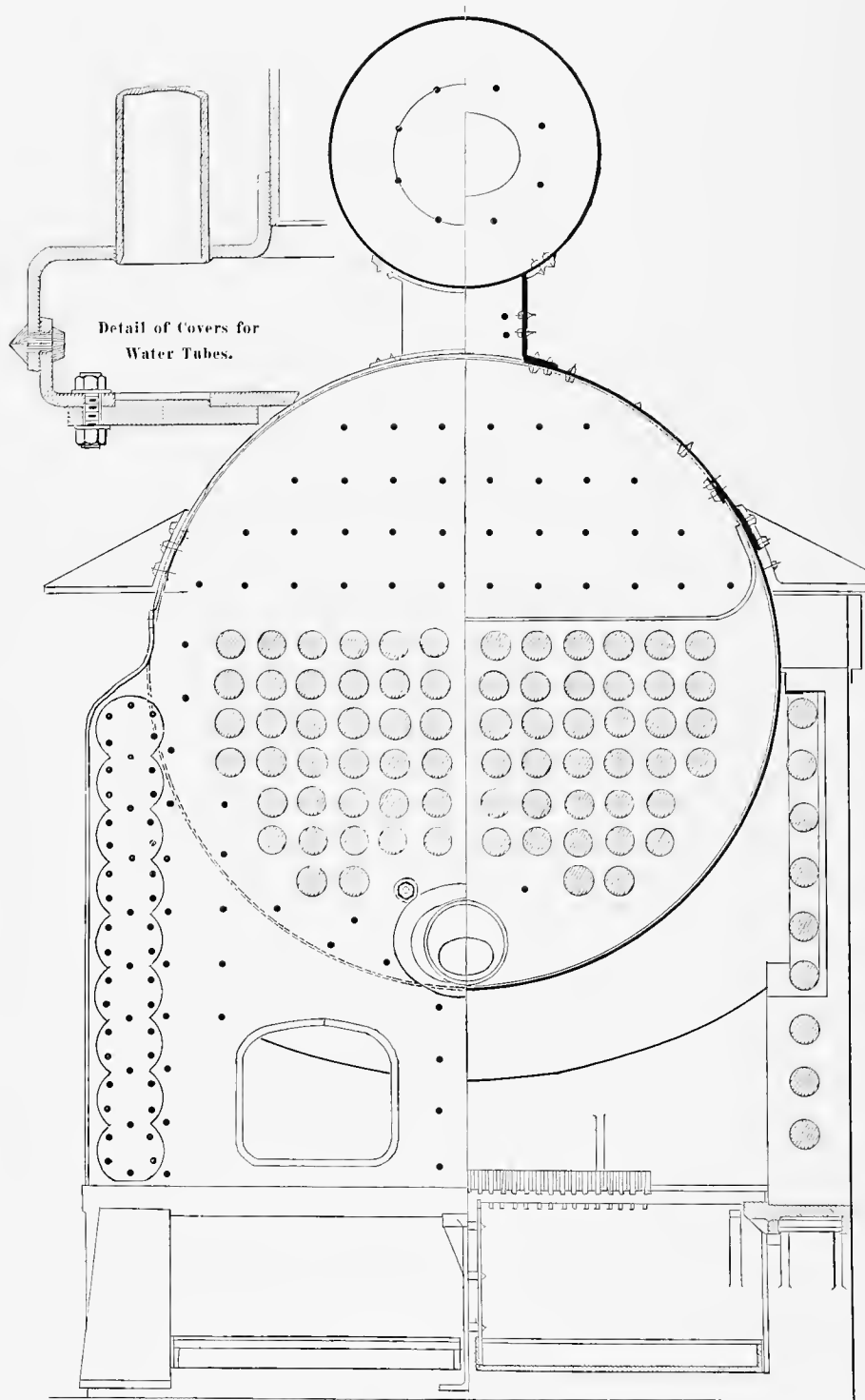
SLOAT'S FIRE AND WATER-TUBE BOILER.
